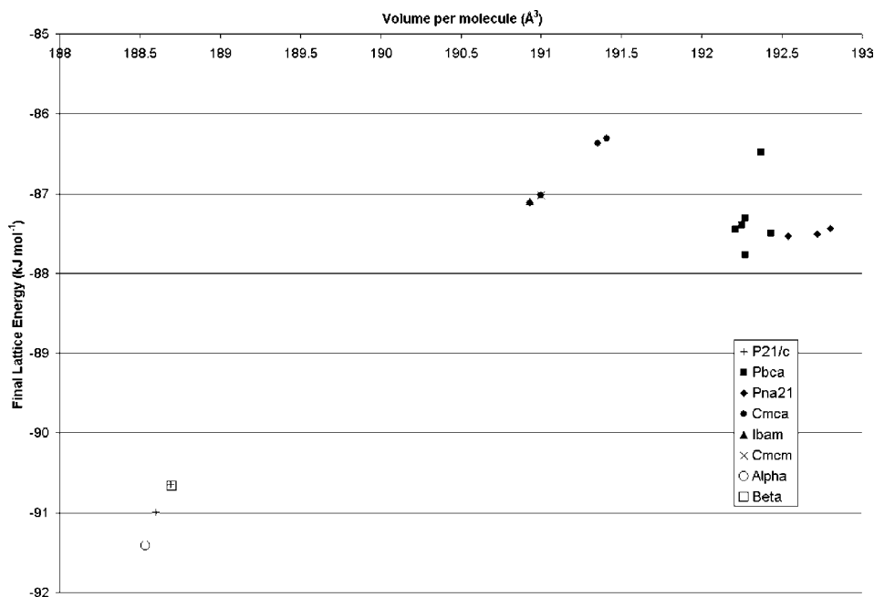
Figure 9 Plot of lattice energy against cell volume per molecule for the unique structures within 5 \text{ kJ mol}^{-1} of the global minimum denoted by the space group assigned after being run through the ADDSYM function of PLATON. The structures corresponding to the \alpha and \beta forms using the same computational model are also shown.
