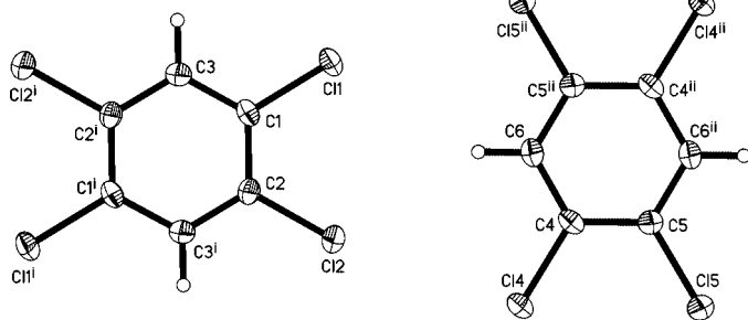
Figure 1 The numbering scheme used for the \alpha form of 1,2,4,5-tetrachlorobenzene. Displacement ellipsoids drawn at the 50% probability level. Symmetry codes: (i) -x, 1 - y, 1 - z ; (ii) 1 - x, -y, -z .
